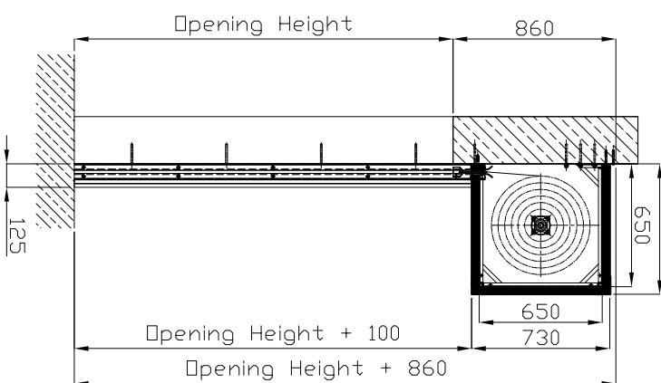
Type 5 housing.
