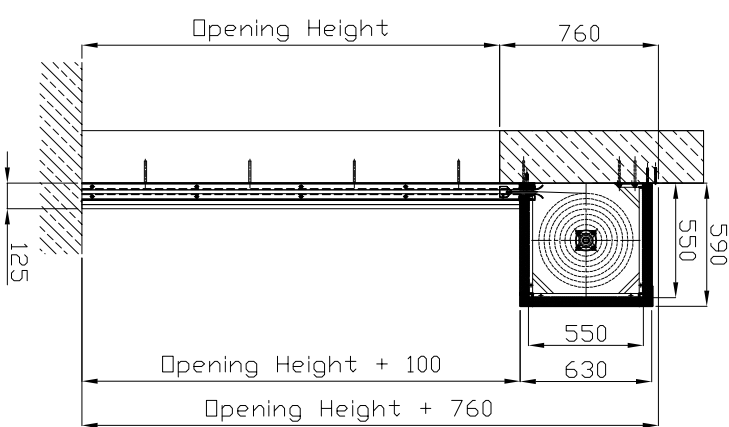
Type 3 housing.
