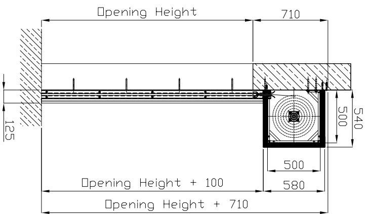
Type 2 housing.
