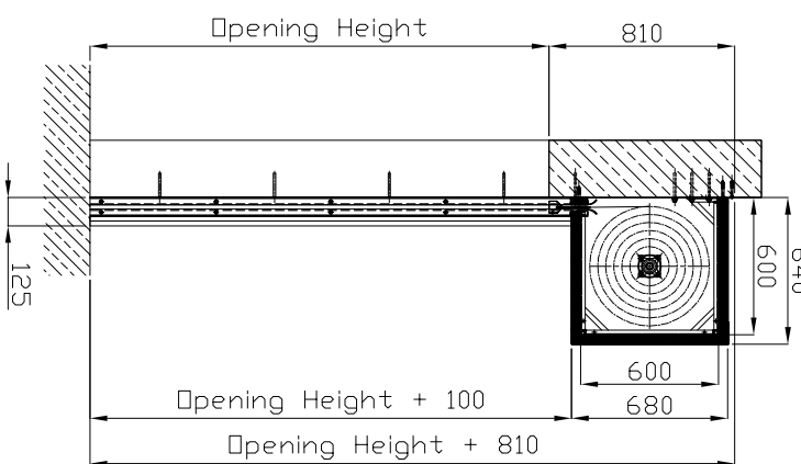
Type 4 housing.
